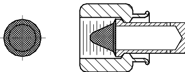
Nozzle Strainer Detail
